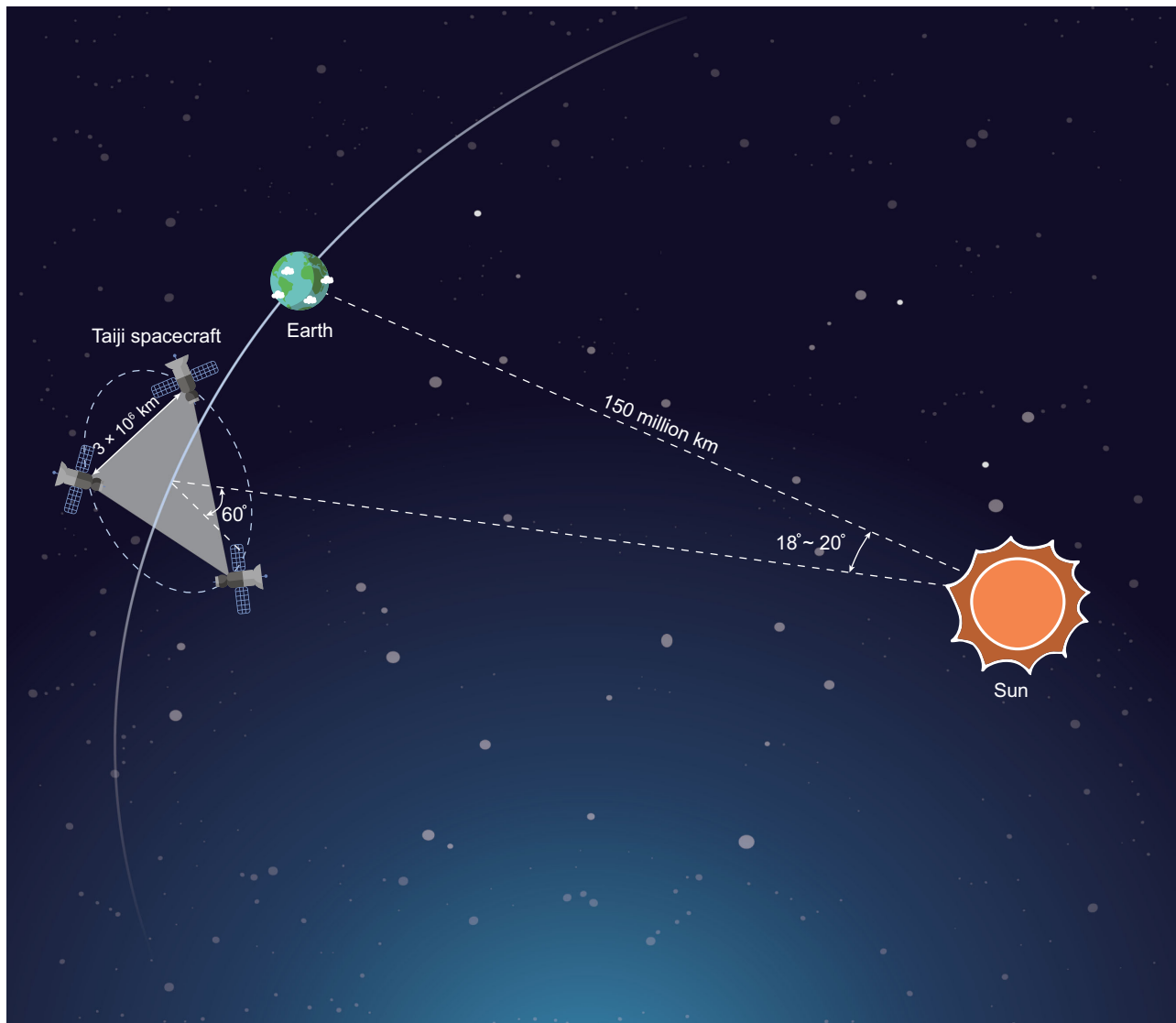
Figure 1. Taiji spacecraft in orbit around the Sun.
